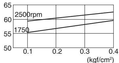
dB(A) TSS-20
