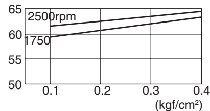
dB(A) TSS-32
