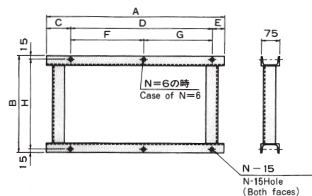
Vibration-isolating Base(SSR)
