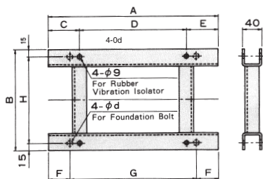
Vibration-isolating Base (TSS,TSA)
