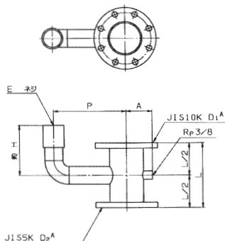
Y shaped reducer (YSS)
