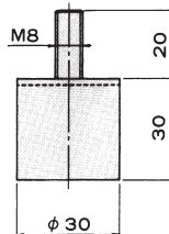
Rubber Vibration Isolator (TSS)
