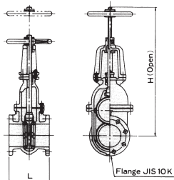
Gate Valve (GV)
