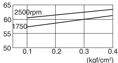
dB(A) TSS-25
