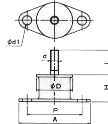
Rubber Vibration Isolator (TYPE B)
