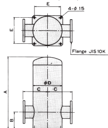
Vertical Discharge Silencer (RKM)
