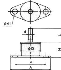
Rubber Vibration Isolator (TYPE B)
