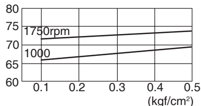
dB(A) TSA-50
