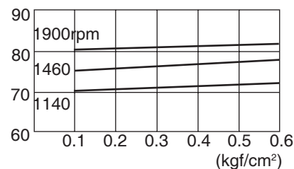
dB(A) SSR-80
