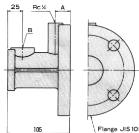
Flange Reducer (TSA)
