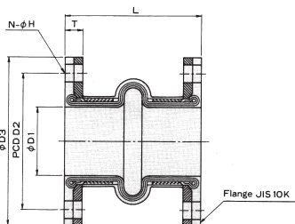
Expansion Joint (EXJ)
