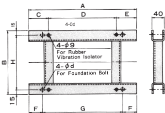
Vibration-Isolating Base (TSS, TSA)
