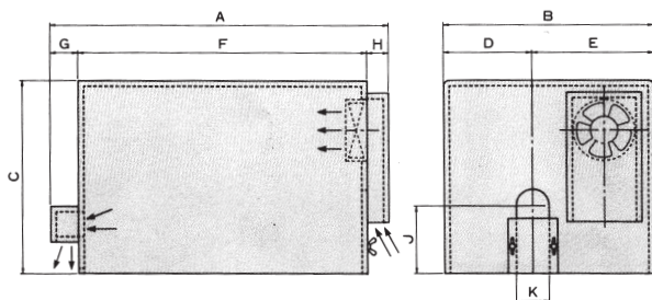
Silencer Box (With Fan)
