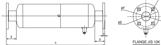
Discharge Silencer (KM)
