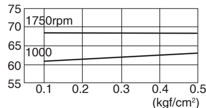
dB(A) TSA-40
