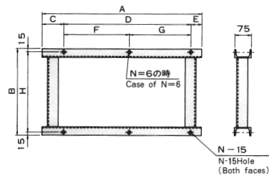
Vibration-Isolating Base (SSR)
