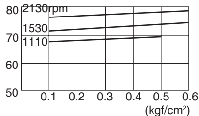
dB(A) SSR-65
